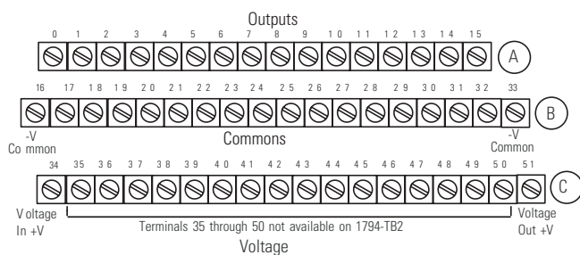
1794-TB2, -TB3, -TB3K and -TB3S
