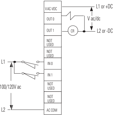
100/120V ac Input - Relay Output
