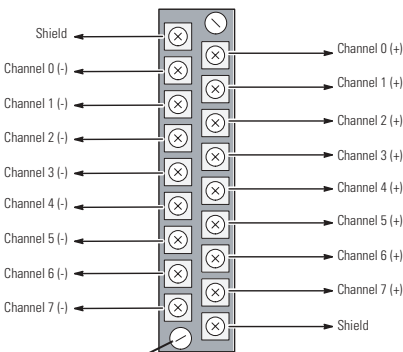
Terminal Block Spare Part Catalog Number 1746-RT25G
