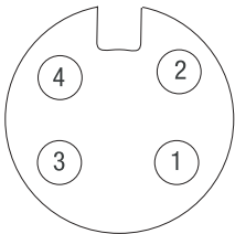
DeviceNet Auxiliary Power
