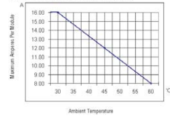
1769-OB32 Maximum Amperes per Module vs. Temperature
