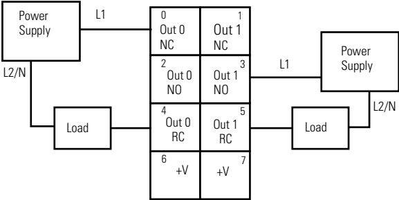
1734-OX2 Load Powered by External Power Bus
