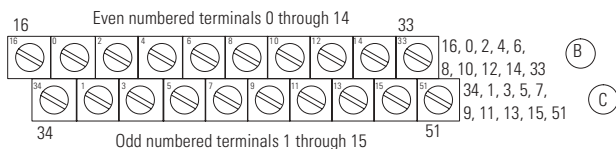
1794-TBN, -TBNK, -TBNF
