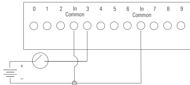
Inputs Sinking
