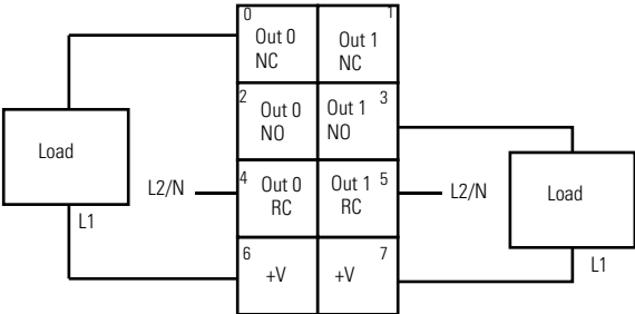
1734-OX2 Load Powered by Internal Power Bus
