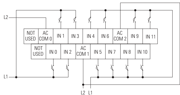
Input Terminals
