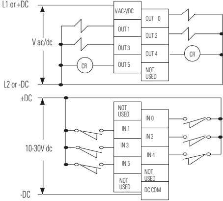
24V dc INPUT - RELAY OUTPUT
