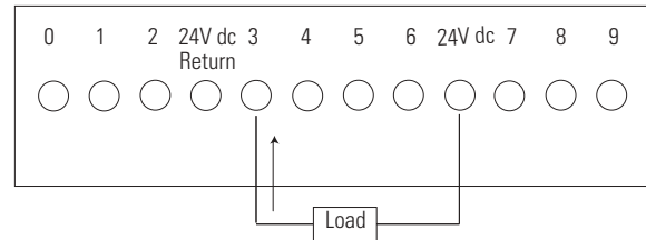
1799-D10U10V, 1799-D10U10VL, 1799-D10U10VZC, 1799-ZCI0V Outputs Sinking
