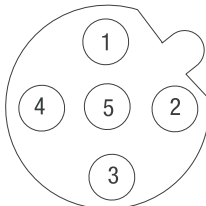
Female In Connector
