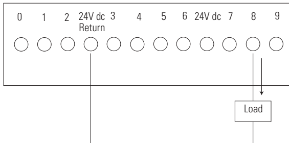
1799-D10U10B, 1799-D10U10BL, 1799-D10U10BZC, 1799-ZCI0B Outputs Sourcing
