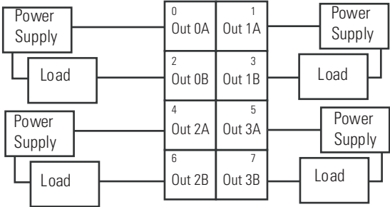
1734-OW4 Load Powered by External Power Bus
