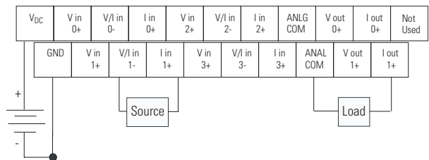
1791D-N4CV2X – Current
