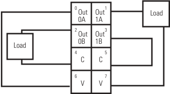
1734-OW2 Load Powered by Internal Power Bus
